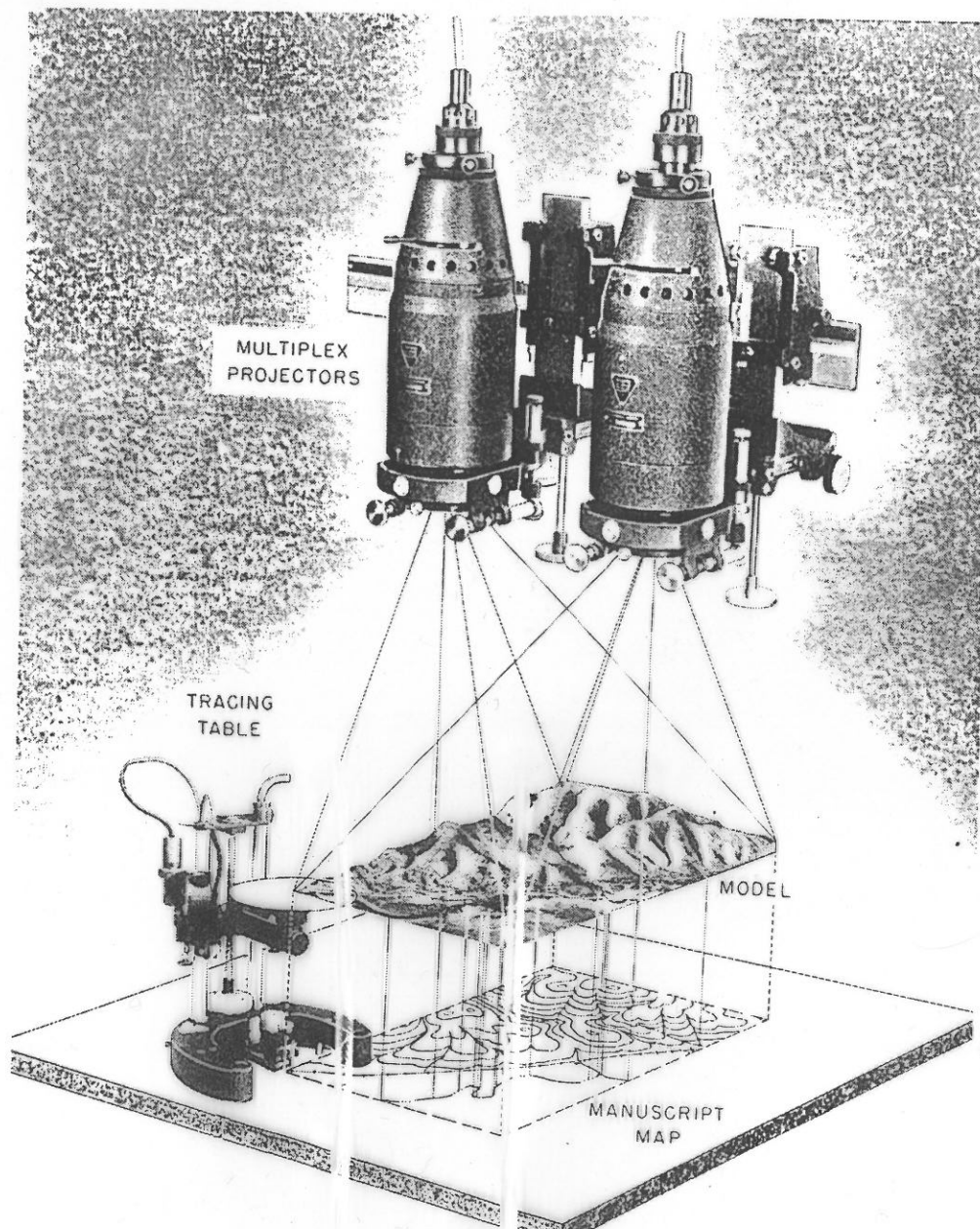
Figure 11-1. Elementary stereoscopic plotting instrument. Bausch and Lomb Multiplex. Courtesy of US Geological Survey.
